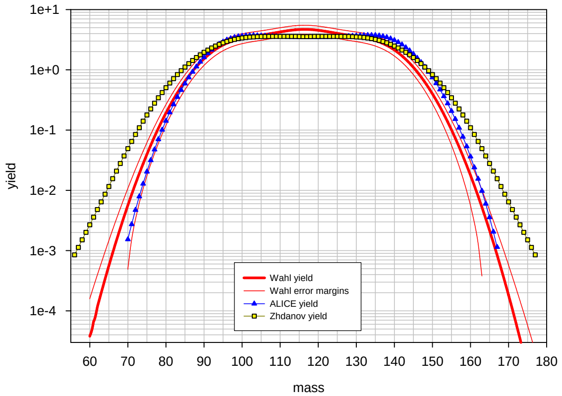
Benchmark B: ^{237}\text{Np} at 100 MeV, pre-neutron emission mass distribution
